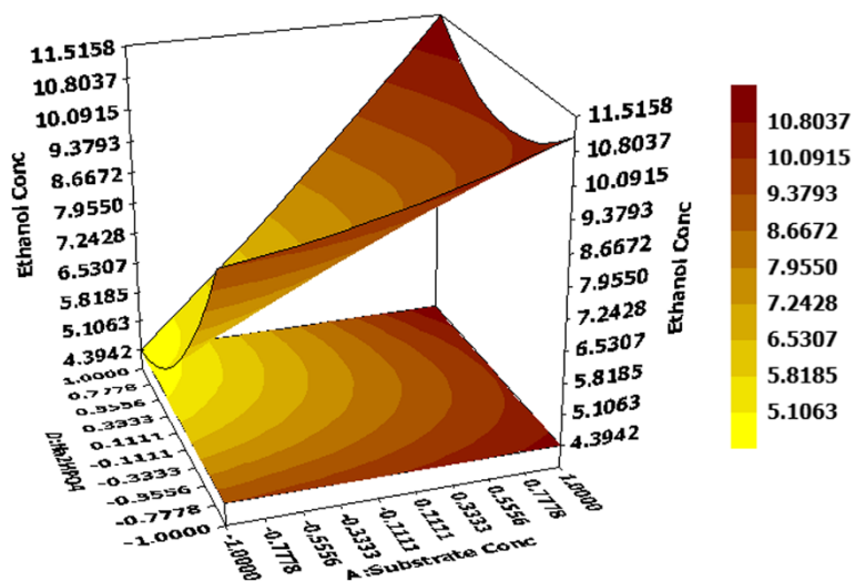
Figure 4 Effects of substrate concentration and Na 2 HPO 4 concentration on ethanol production hold values: B = 0 (pH = 5.0), C = 0 (fermentation time = 36 hours).
