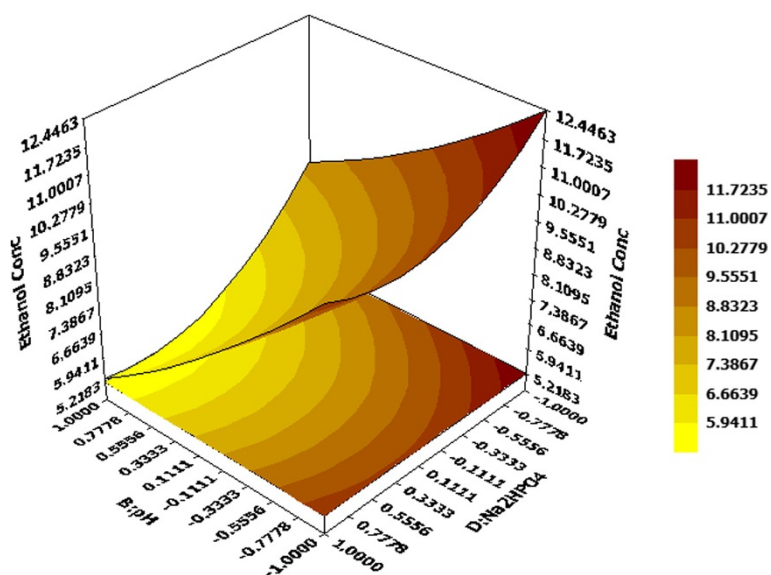
Figure 3 Effects of pH and Na 2 HPO 4 concentration on ethanol production hold values: A = 0 (substrate Conc. = 30 g/L), C = 0 (fermentation time = 36 h).
